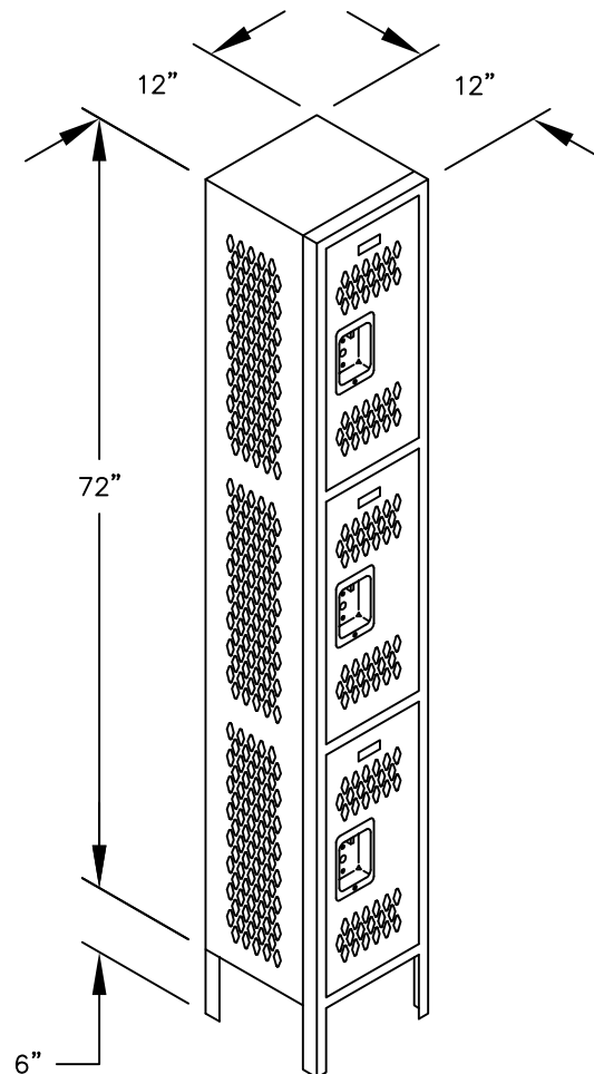
MODEL #73162 TRIPLE TIER VENTED LOCKER — 1 WIDE
