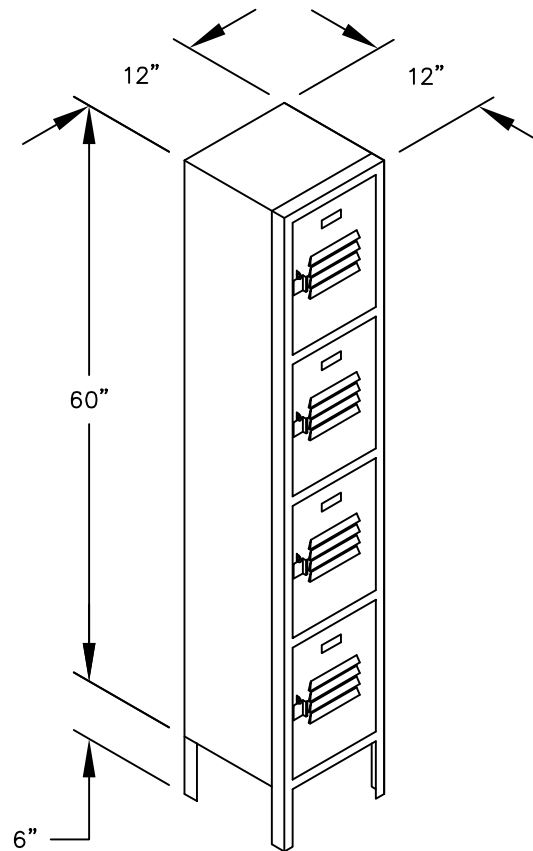
MODEL #64152 FOUR TIER STANDARD LOCKER — 1 WIDE
