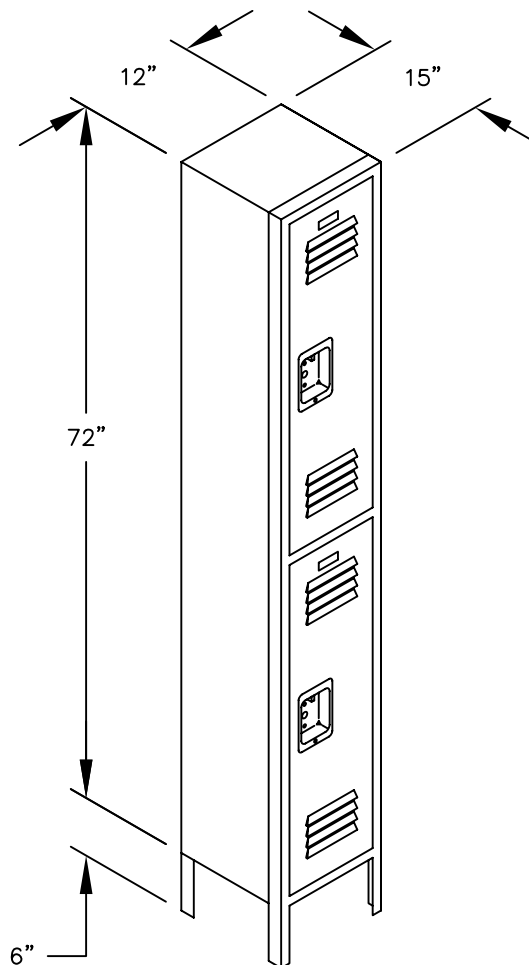
MODEL #62165 DOUBLE TIER STANDARD LOCKER — 1 WIDE
